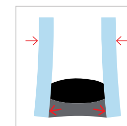
Contracted IGU
