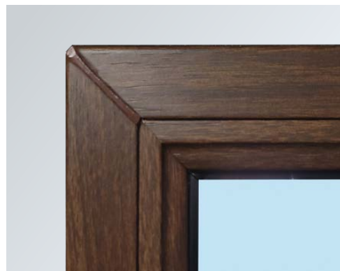
Fusion welded mitered corners
